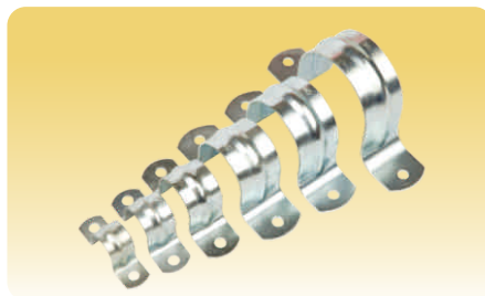
Part No.:DXM012 Full saddle 16, 20, 25, 32, 40, 50mm Eg: DXMO12/16
