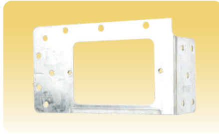
Part No.:DXM010 1.0mm vertical/horizontal mounting stud bracket
