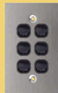
Part No.:DXSSW5V/B Heavy duty stainless steel 16amp five gang two way switch, black, vertical
